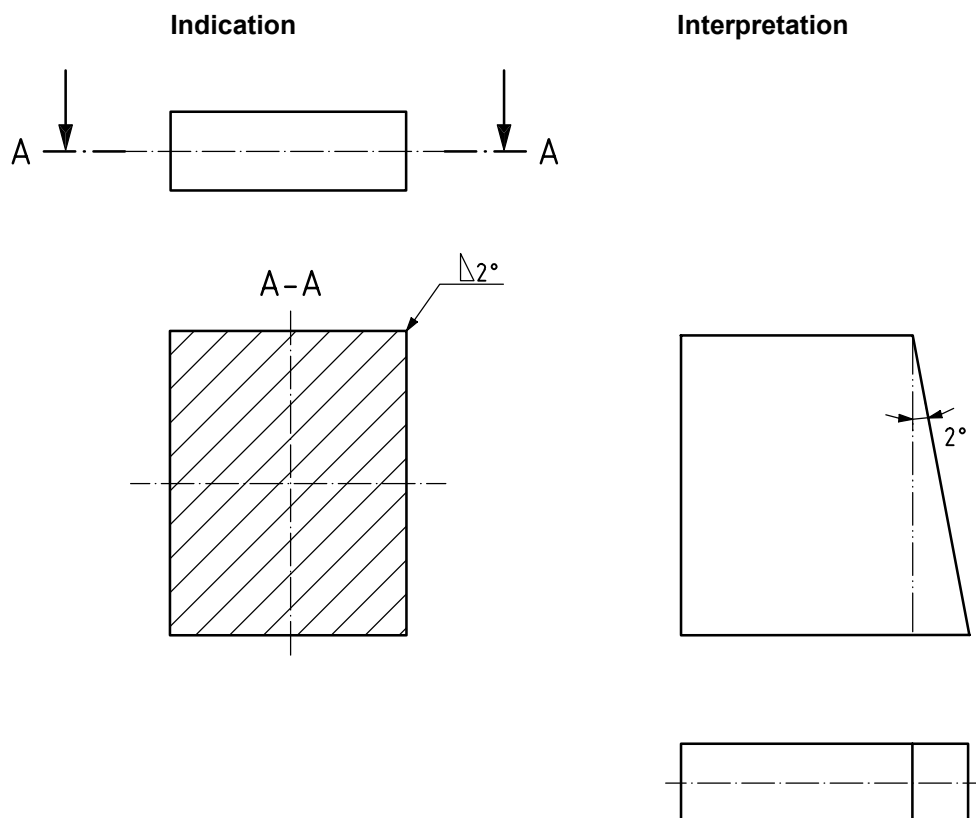
Figure 79 — Draft angle indication on a feature represented on a cross section of a part
