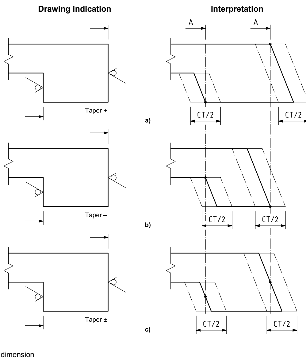
Figure B.1 — Tolerance zone on tapered features
