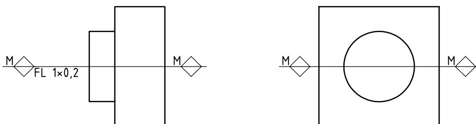
Figure 31 — Example of an indication of global requirement of flash
