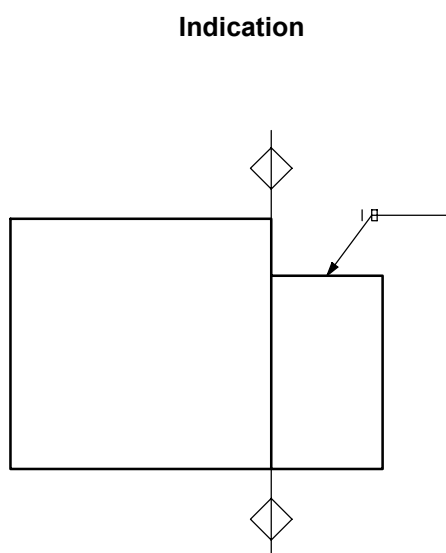
Figure 53 — Partial all about symbol on leader and reference lines used with horizontal axis indicator
