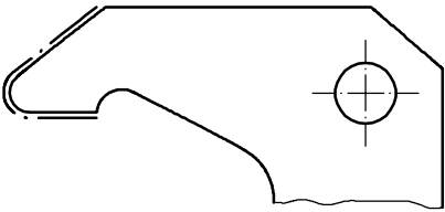
Figure 38 — Indication of a combination of adjoining features
