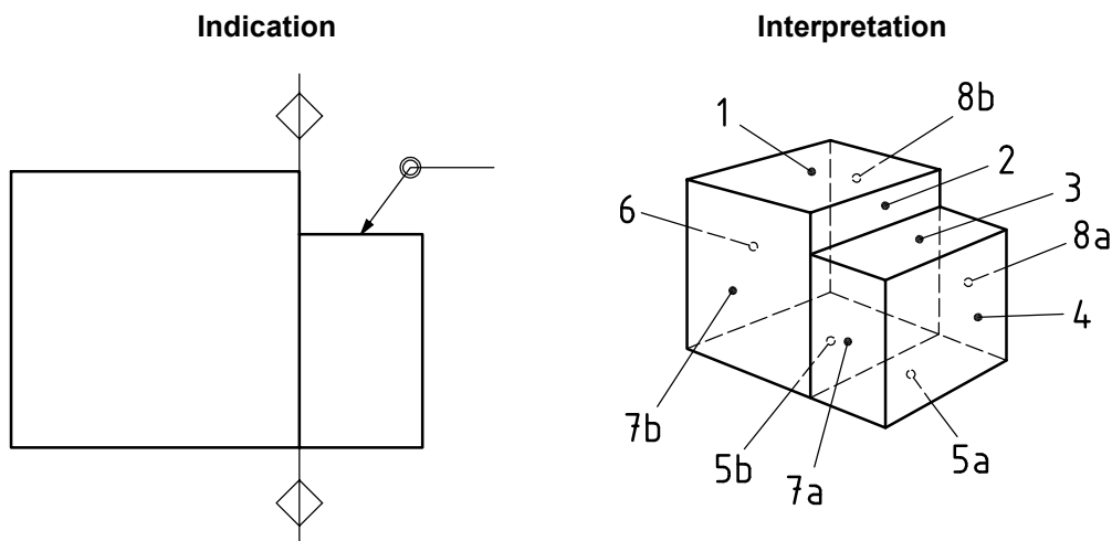
Figure 56 — Graphical symbol for indication of global all over condition used on leader and reference lines
