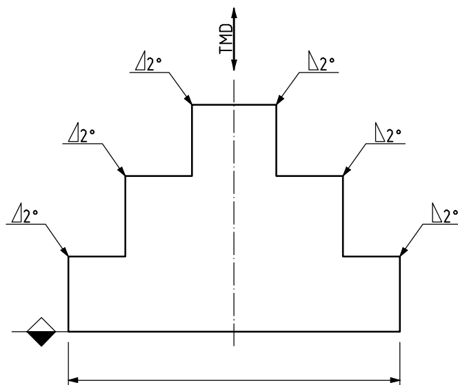
Figure 85 — Example of the indication of tool motion direction
