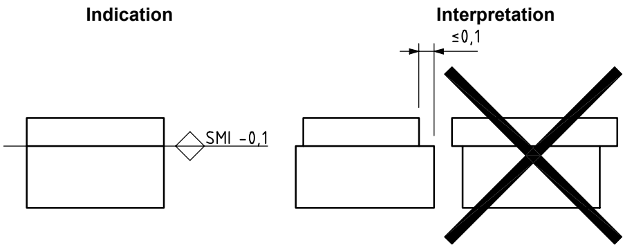
a) Permissible surface mismatch with + (plus) sign
