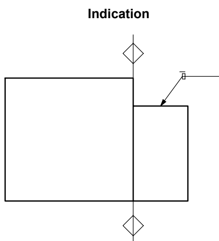
Figure 52 — Graphical symbol for indication of partial all about condition used on leader and reference lines
