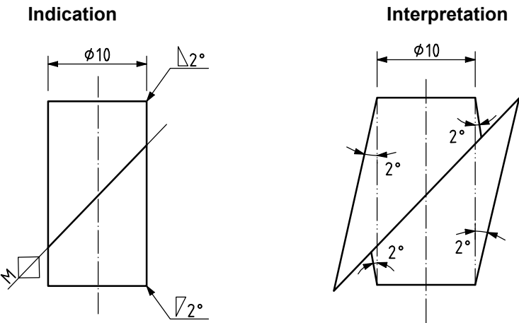
Figure 70 — Inclined parting surface on a part with a numerical specified draft
